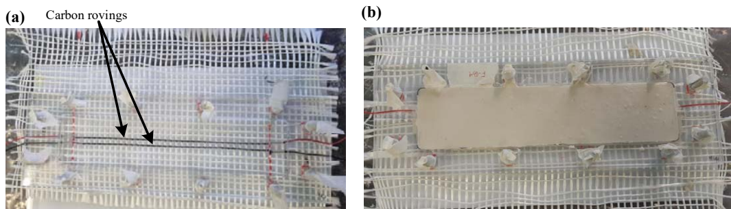
Figure 1. Beam specimen in the mold: (a) Before casting, (b) After casting.
