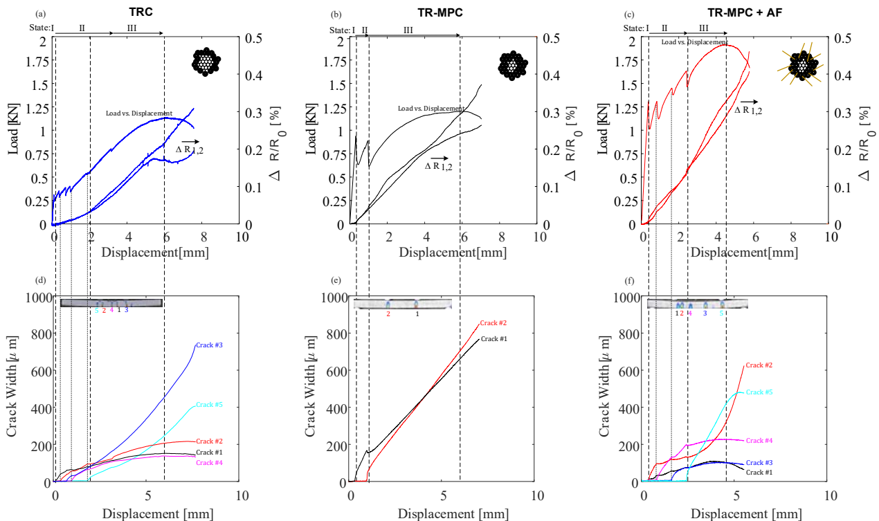
Figure 3. Structural and electrical response of TRC, TR-MPC and TR-MPC +AF: (a-c) load vs. displacement and ERC of the carbon rovings, (d-f) crack formation and propagation analysis.
