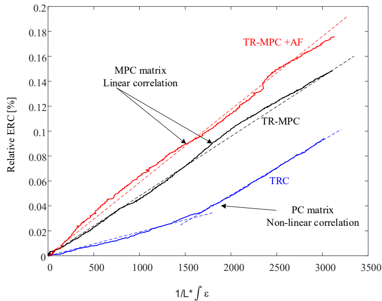
Figure 4. Comparison of the composites structural-electrical correlation: Linear correlation of MPC matrices and nonlinear correlation PC matrix
