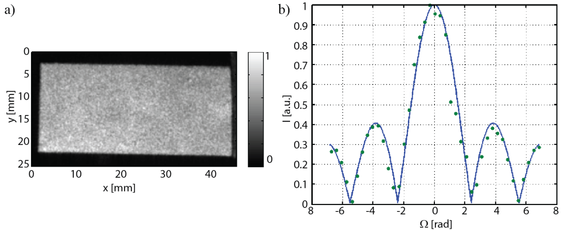
Fig. 2: a) Reconstructed intensity image of steady-state object with no phase modulation \Omega = 0 ; b) measured (green) and fitted (blue) intensity values at x = 25 mm and y = 13 mm as a function of the modulation depth
